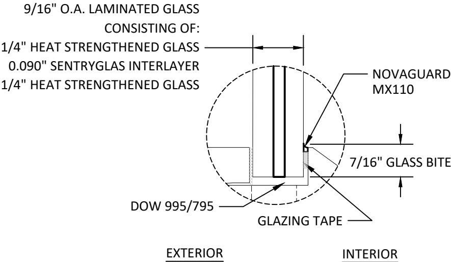
GLAZING DETAIL 1
