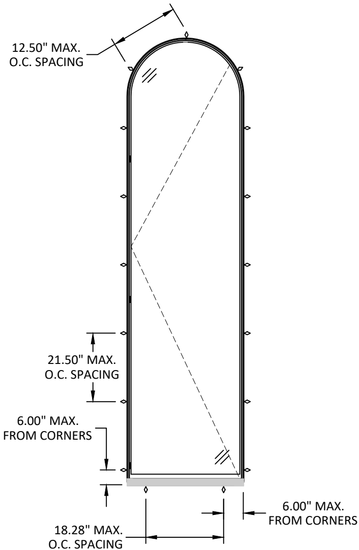
ANCHOR LAYOUT THROUGH FRAME / ALUMINUM ANGLE / HRS12 STRAP INSTALLATION
