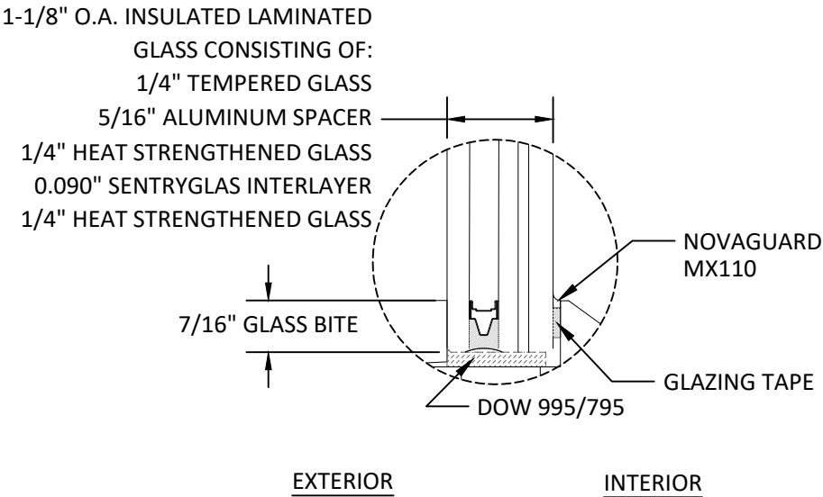
GLAZING DETAIL2
