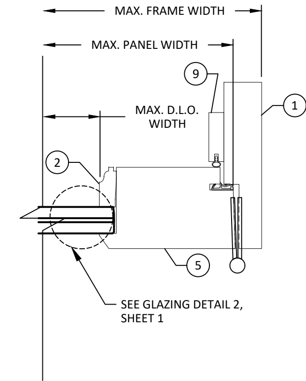
C 12 HORIZONTAL SECTION TYP. HINGE JAMB DETAIL
