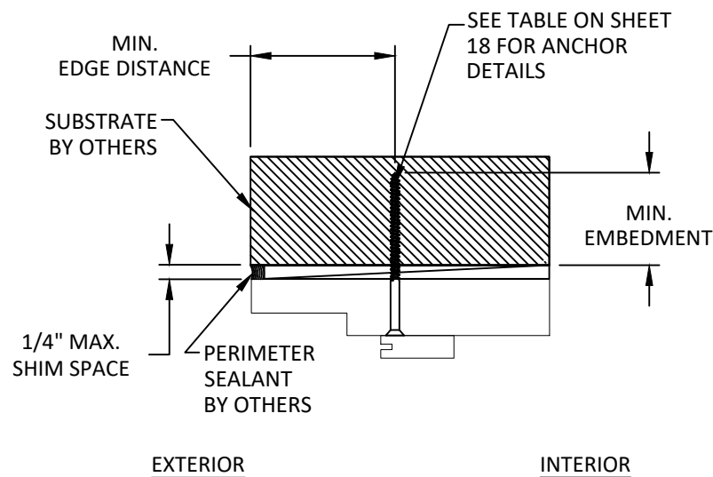
D 16 VERTICAL SECTION THROUGH FRAME - HEAD SHOWN, JAMB/SILL SIMILAR
