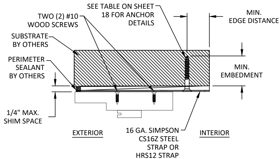
A 16 VERTICAL SECTION STRAP - HEAD SHOWN, JAMB/SILL SIMILAR
